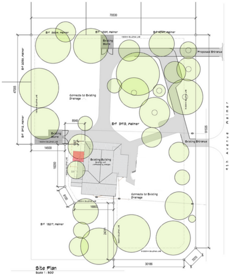
Property Layout
